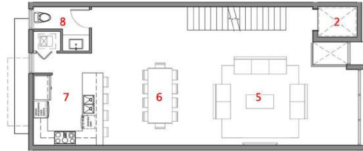
2ND FLOOR
