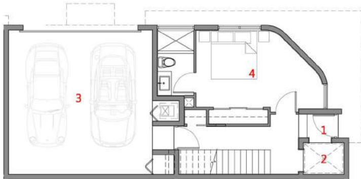
1ST FLOOR
