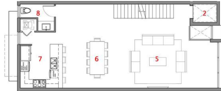
2ND FLOOR
