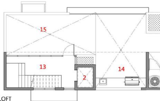
ROOF LOFT
